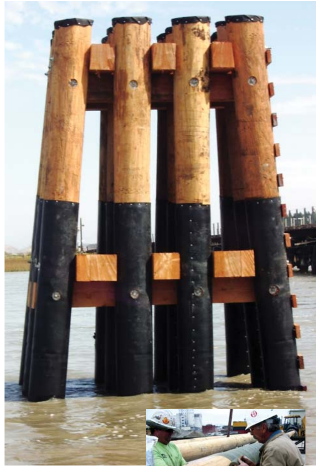
SeaShield Series 90 consists of SeaShield Marine Tape preventing marine borer destruction and an outercover for mechanical protection of tape.
