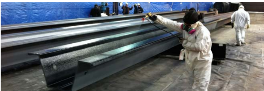
Denso Rigspray being applied to steel sheet piles with an airless spray unit.
