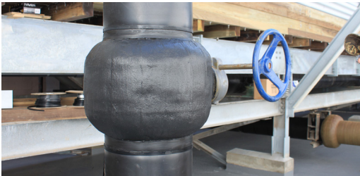
Weathershield 15 brushed applied onto Densyl Tape protecting a valve flanged as a top coat.
