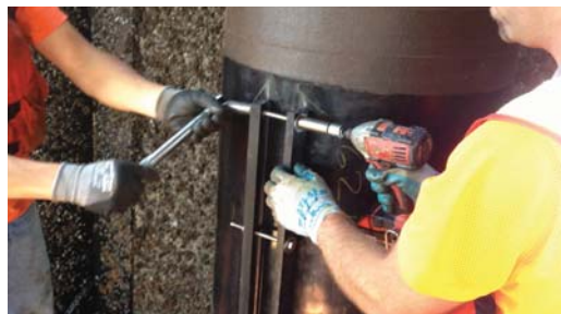
Installing the 80 mil HDPE outercover with M10 316SS fasteners.
