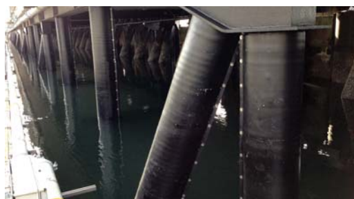
Completed piles fully protected with the SeaShield Series 2000HD System.
