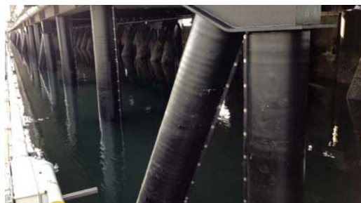
Completed piles fully protected with the SeaShield Series 2000HD System.
