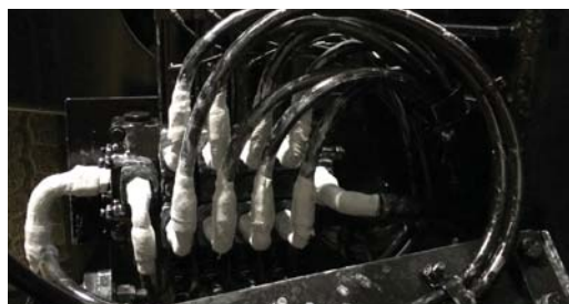
Hydraulic hose fittings protected with Denso ColorTape against harsh weather conditions and water infiltration.
