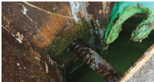
Denso Hi-Tack Paste is first applied to the tie rod to displace moisture and prevent rusting.
